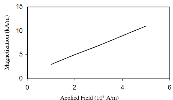
Fig. 1 Magnetization as a function of applied field.
